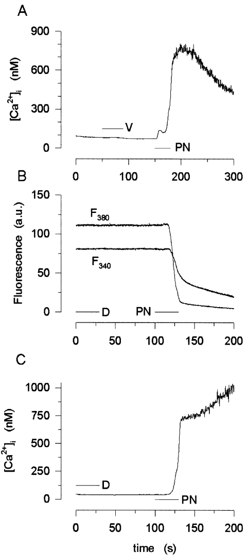
Figure 4. The effect of peroxyntirite (PN, 10 \mu M), decomposed PN (D), or the vehicle (V, see Materials and Methods) on [Ca^{2+}]_i . (A) The vehicle and peroxyntirite were applied subsequently (for 40 and 30 s, respectively) as indicated. Note that whereas the vehicle had no measurable effect peroxyntirite caused a substantial increase in [Ca^{2+}]_i . (B) Peroxyntirite caused a non-specific increase in membrane permeability indicated here as a drop in fluorescence (arbitrary units, a.u.), both at 340 and 380 nm. (C) Changes in [Ca^{2+}]_i calculated from the fluorescence signals shown in panel B. Note the increase in noise (in A and C) that is attributed to the low fluorescence levels in these cells after the application of peroxyntirite. Data are presented from two different cells, representative of 13 experiments. Statistical analysis (Student's paired t test) showed that neither vehicle nor decomposed peroxyntirite caused significant elevation in intracellular calcium ( p > 0.08 for vehicle, p > 0.11 for decomposed peroxyntirite). Peroxyntirite-induced elevation in intracellular calcium was statistically significant ( p < 0.04 ). (Note that in some peroxyntirite-treated cells, calcium level reached micromolar range where saturation of the dye makes the measurement less accurate. Omission of these cells from the statistical evaluation results in a higher degree of significance: p < 0.003 ).
