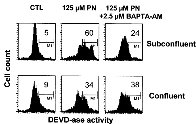
Figure 8. Effect of BAPTA-AM and cell density on peroxyntirite-induced caspase activation. Subconfluent (80%) and confluent (100%) HaCaT cells were treated with peroxyntirite in the presence or absence of BAPTA-AM (2.5 \mu M). After 6 h cells were stained with the fluorogenic PhiPhiLux caspase-3 substrate and analyzed by flow cytometry. Caspase activation is indicated by increased fluorescence (right shift). Numbers indicate the percentage of cells displaying increased fluorescence (caspase activation).
